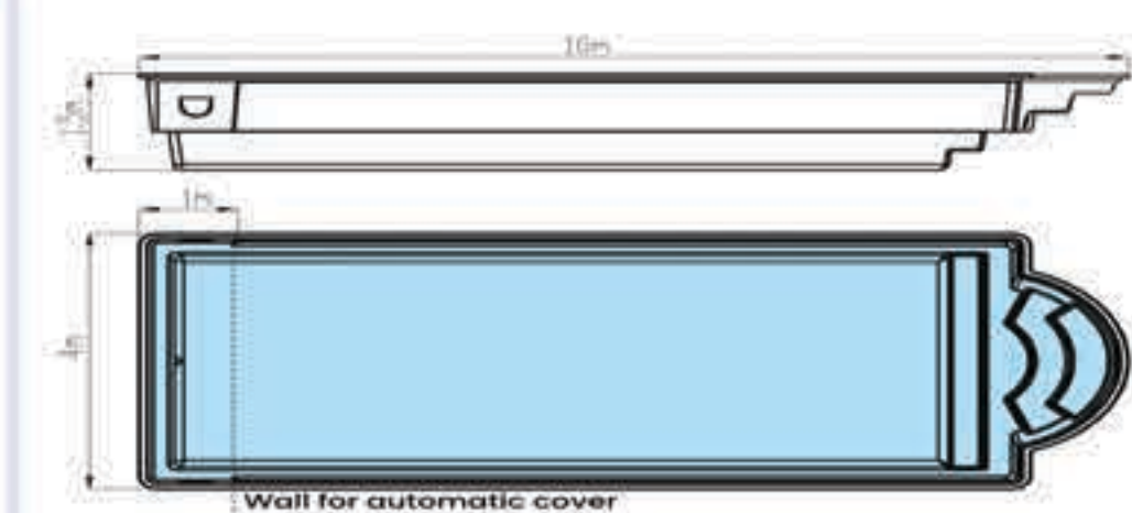
GOLF 10 X 4 X 1.5 R/N/C
