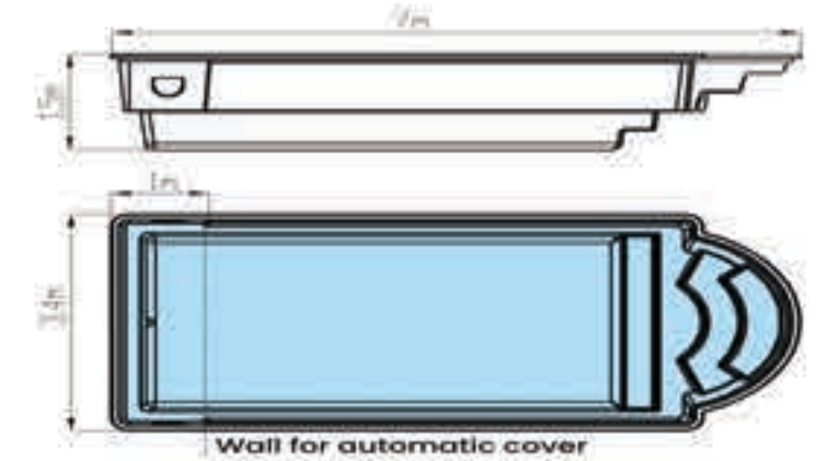
GOLF 8 X 4 X 1.5 R/N/C
