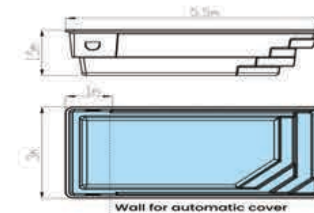
DELTA 5.5 X 3 X 1.5 R/N/C
