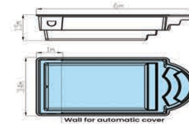
GOLF 8 X 3.6 X 1.5 R/N/C
