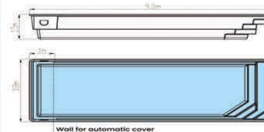
DELTA 9.5 X 3.8 X 1.5 R/N/C
