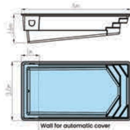
MARINA 8 X 3.6 X 1.1 - 1.8 R/N/C
