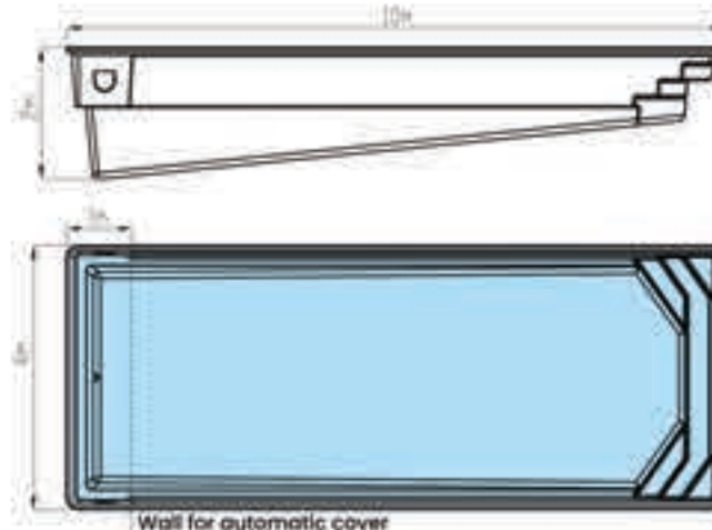
MARINA 10 X 4 X 1.1 - 2.0 R/N/C
